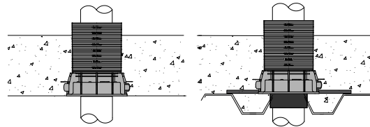
CID Alignment connectors allow tight placement of multiple penetrations.
