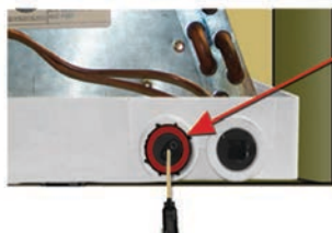
Probe Sensor (Mounted to Side of Unit)
